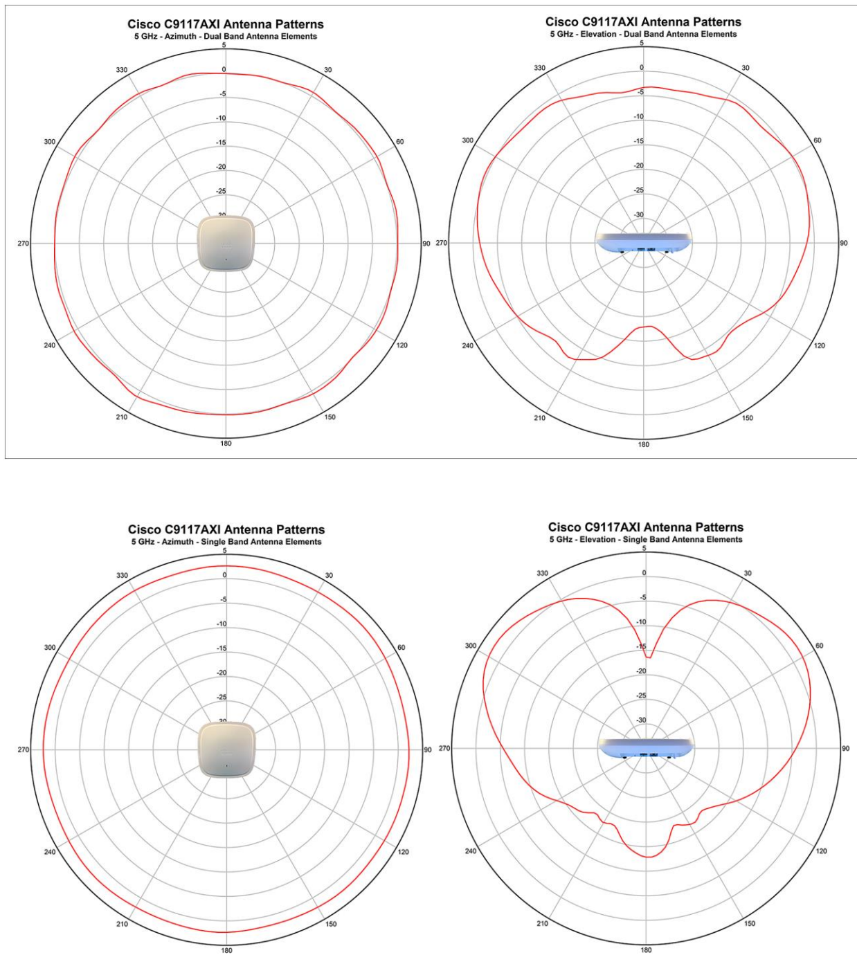
Figure 2. Antenna radiation patterns for the 9117AXI
